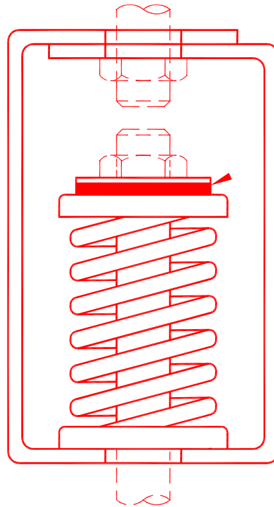
SHS-13 (Spring Hanger)
