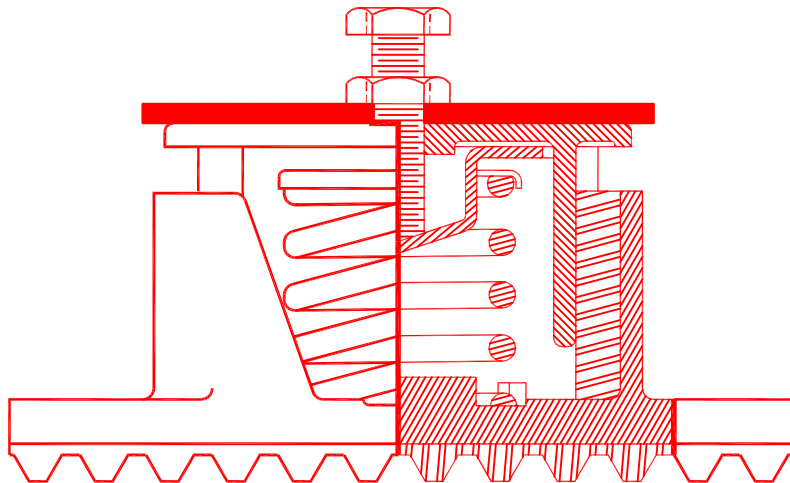
BE-12 (Spring Mount)
